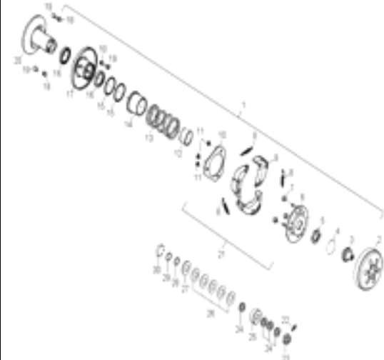
D-9: DRIVEN CLUTCH
