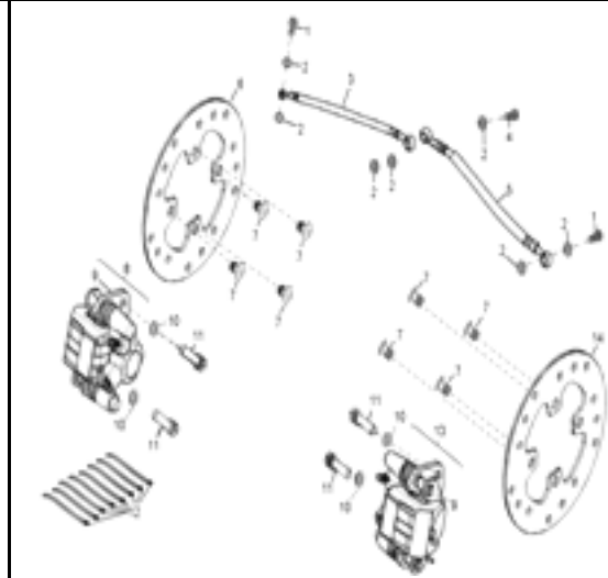
D-26: FRONT BRAKE
