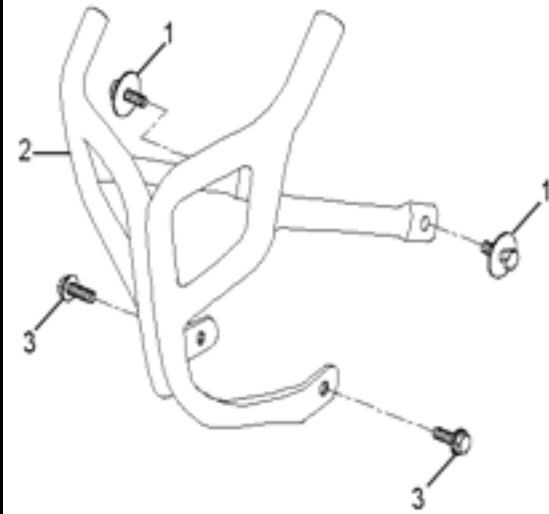
D-19: BUMPER
