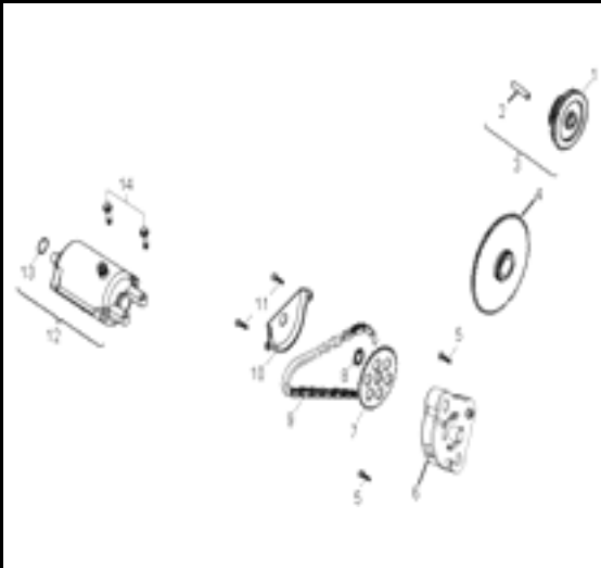
D-10: OIL PUMP & STARTING MOTOR
