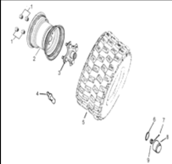
D-25: REAR WHEEL
