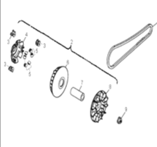
D-8: DRIVE CLUTCH
