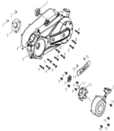
D-5: LEFT CRANKCASE COVER
