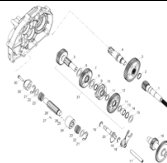
D-11: TRANSMISSION
