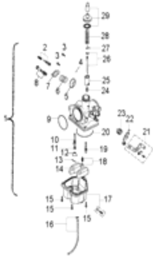
D-13: CARBURETOR
